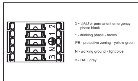
3. Electrical connection of terminal block 5.pol.
