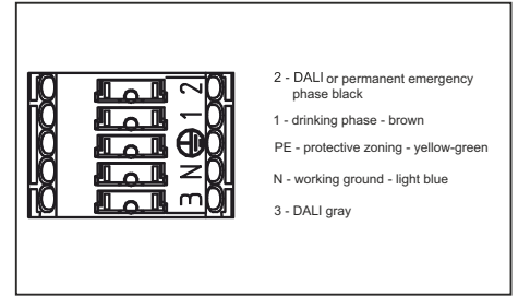
3. Electrical connection of terminal block 5.pol.
